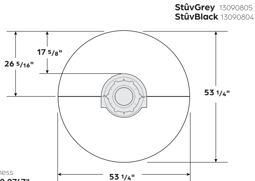
FP4 – Rotation 360°
